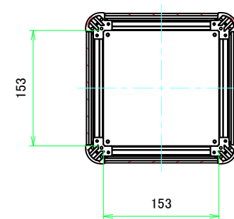
C-C (1:5)
